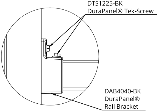
Panel Bracket Detail 1:3
