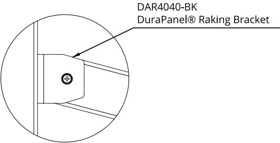
Raking Panel Bracket Detail 1:3
