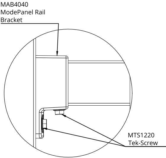
Panel Bracket Detail 1:2
