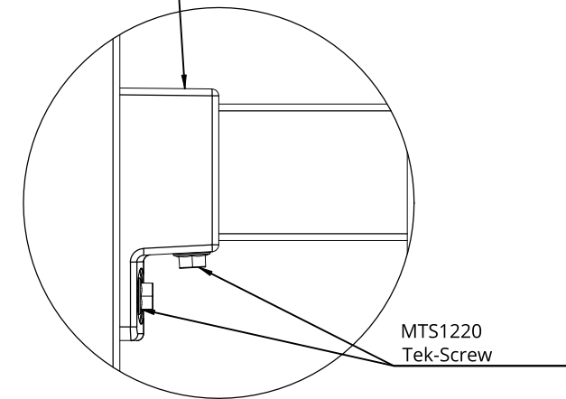
Panel Bracket Detail 1:2
