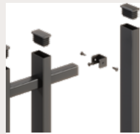
Top Fixing
