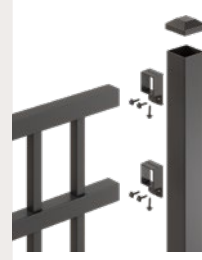
Top Fixing
